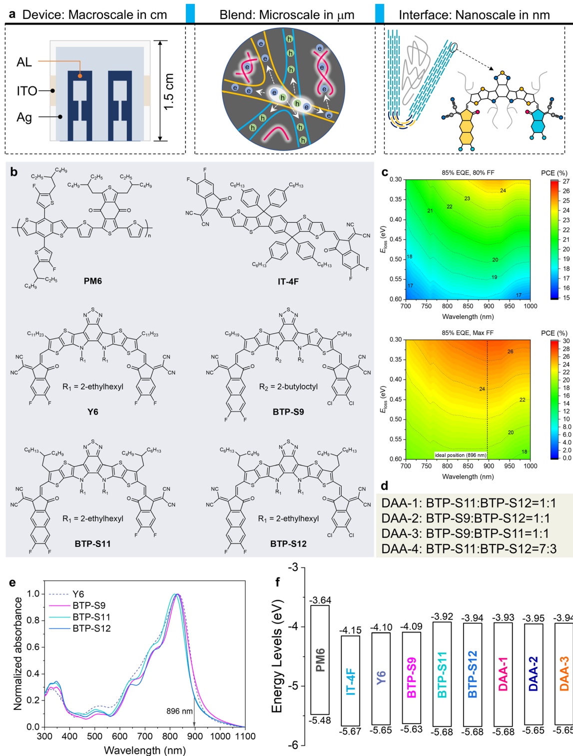
Fig. 1 (a) Schematics of various research studies in macroscale (constructing island-like electrode for single device), microscale (double-fibril network morphology for charge separation and transport in ternary blend; blue fibril is donor, yellow fibril is acceptor, red fibril is third component) and nanoscale (straight-crystal and curved-crystal arrangements at the D–A interfaces) levels. (b) Molecular structures of PM6, IT-4F, Y6, BTP-S9, BTP-S11 and BTP-S12. (c) Theoretical calculations of power conversion efficiencies for single-junction OPVs with the sets of 85% EQE and 80% FF/max FF. (d) Illustrations of DAA-1, DAA-2, DAA-3 and DAA-4. (e) Normalized absorption spectra of Y6, BTP-S9, BTP-S11 and BTP-S12 films. (f) Energy level diagrams of materials studied in this work.
