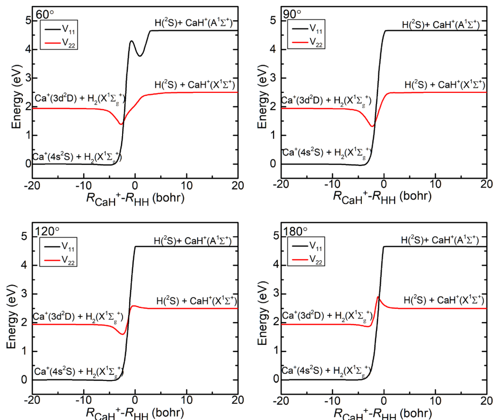
Fig. 2 Minimum energy paths of V_{11}^{41} and V_{22}^{22} for the Ca-H-H angle fixed at 60.0°, 90.0°, 120.0° and 180.0°.
