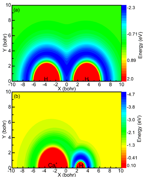
Fig. 3 (a) Contour plot for a \text{Ca}^+ ion moving around a \text{HH} molecule fixed at R_{\text{HH}} = 7.32 bohr and lying along the x-axis. (b) Color plot for a \text{H} atom moving around a \text{CaH}^+ molecule ion fixed at R_{\text{CaH}} = 5.06 bohr. The dissociation limit of the \text{CaH}_2^+ molecule ion is set as the zero point of potential energy.
