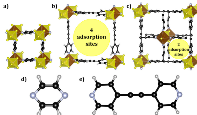
Fig. 1 Pore structure for (a) SIFSIX-3-Cu, (b) SIFSIX-2-Cu, (c) SIFSIX-2-Cu-i, and the organic linkers (d) pyrazine and (e) 4,4'-dipyridylacetylene. The colors corresponding to each atom are carbon (black), hydrogen (grey), nitrogen (blue), fluorine (yellow) and copper (brown).
