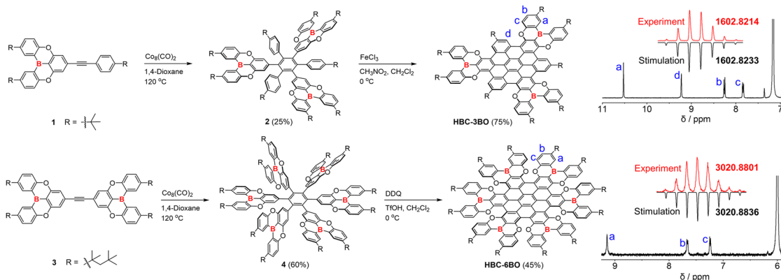
Scheme 1 Synthesis of HBC-3BO and HBC-6BO . Insets are their HRMS and ^1\text{H} NMR spectra.
