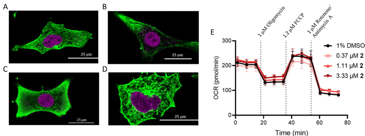
Fig. 4 Excluded mechanisms of action. Tubulin polymerization was measured in (A) untreated A549 cells and cells treated with 1 \mu\text{M} compounds: (B) paclitaxel, (C) vinblastine, and (D) 2. The cells were incubated with each compound for 16 h. (E) Mitochondrial stress was evaluated following treatment with increasing concentrations 2 at 1 h.
