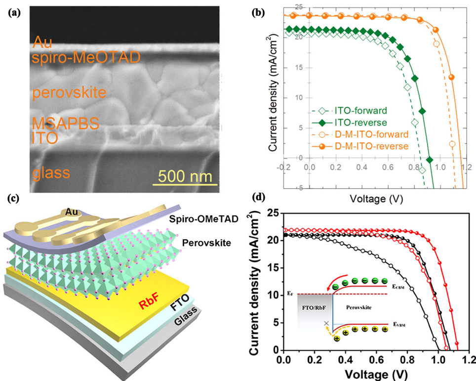
Fig. 4 (a) Cross-sectional SEM image and (b) J - V curves of PSCs for the bottom electrode/perovskite interface of normal structural PSCs based on MSAPBS. Reproduced with permission from ref. 56. Copyright 2020 Wiley. (c) Device structure diagram and (d) J - V curves of PSCs for the bottom electrode/perovskite interface of normal structural PSCs based on RbF. Reproduced with permission from ref. 57. Copyright 2020 Elsevier.
