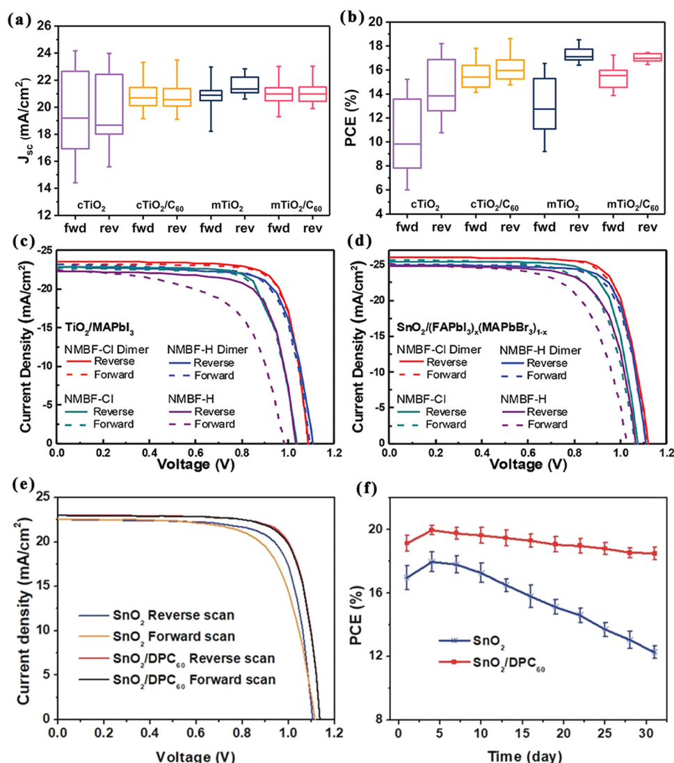
Fig. 6 Fullerene ( \text{C}_{60} ) and derivatives for ETL/perovskite interfaces of normal structured PSCs. (a) and (b) Photovoltaic parameters of \text{C}_{60} -based PSCs. Reproduced with permission from ref. 70. Copyright 2020 American Chemical Society. (c) and (d) J - V curves of PSCs based on \text{TiO}_2 and \text{SnO}_2/\text{NMBF-X} monomers and dimers. Reproduced with permission from ref. 71. Copyright 2020 Wiley. (e) and (f) J - V curves of PSCs based on \text{SnO}_2 and \text{SnO}_2/\text{DPC}_{60} and measured curves of environmental stability. Reproduced with permission from ref. 72. Copyright 2019 Wiley.
