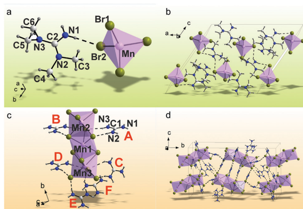
Fig. 1 Crystal asymmetric structure units of (\text{C}_5\text{H}_{14}\text{N}_3)_2\text{MnBr}_4 (a) and (\text{CH}_6\text{N}_3)_2\text{MnBr}_4 (c). The atoms in the asymmetric part of the unit cell (\text{C}_5\text{H}_{14}\text{N}_3)_2\text{MnBr}_4 (b) and (\text{CH}_6\text{N}_3)_2\text{MnBr}_4 (d) are labeled, the hydrogen bonds in which are presented as dashed lines. The independent [\text{CH}_6\text{N}_3]^{2+} cations in the Figure (c) are marked by bold labels A–E.
