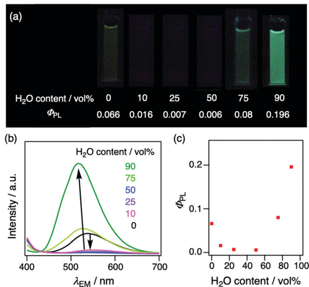
Fig. 5 (a) Photographs taken under blacklight ( \lambda_{\text{EX}} = 365 \text{ nm} ), (b) PL spectra, and (c) plots of absolute \phi_{\text{PL}} against H 2 O content (vol%) in THF solution of 2Cz2SB ( 2 \times 10^{-5} \text{ M} ).
