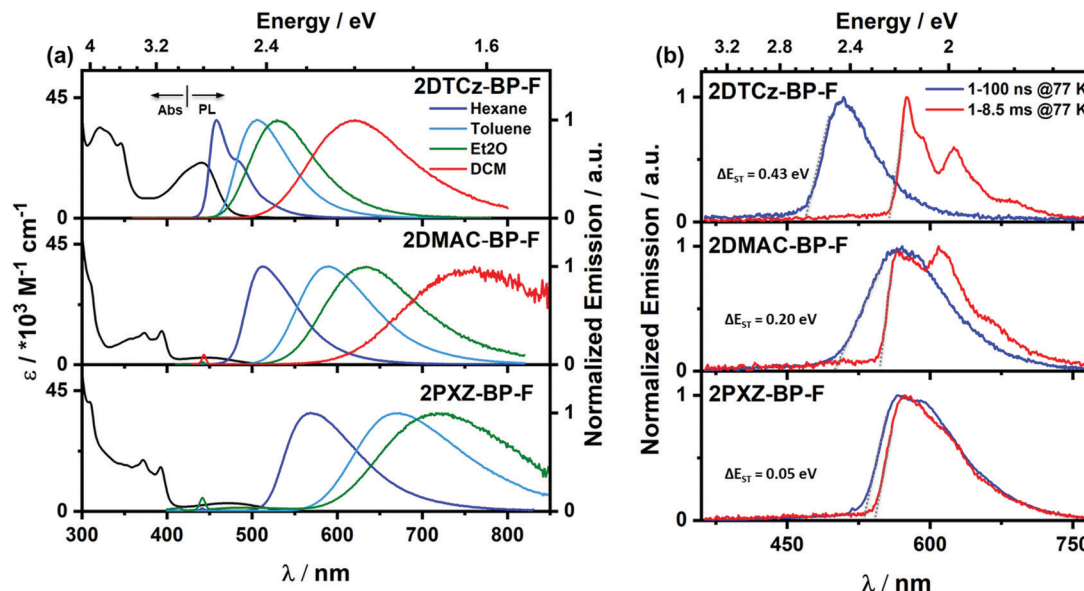
Fig. 5 (a) UV-vis absorption and PL solvatochromism study ( \lambda_{exc} = 343 nm); (b) prompt fluorescence (blue line) and phosphorescence (red line) spectra of 2DTCz-BP-F and 2DMAC-BP-F in 2-MeTHF, 2PXZ-BP-F in hexane at 77 K ( \lambda_{exc} = 343 nm, prompt and delayed fluorescence spectra were obtained in the 1–100 ns and 1–8.5 ms time range, respectively). Et 2 O = diethyl ether; DCM = dichloromethane.
