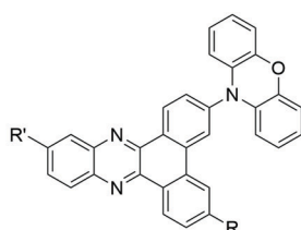
1PXZ-BP: R = R' = H 2PXZ-BP: R = \text{PXZ}, R' = H 3PXZ-BP: R = R' = \text{PXZ}
