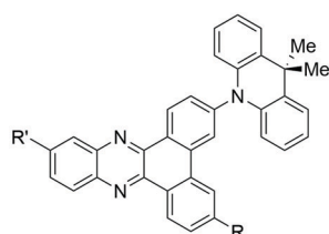
1DMAC-BP: R = R' = H 2DMAC-BP: R = \text{DMAC}, R' = H 3DMAC-BP: R = R' = \text{DMAC}
