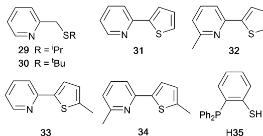
Scheme 13 Structures of chelating \text{N}^{\wedge}\text{S} and \text{P}^{\wedge}\text{S} ligands.
