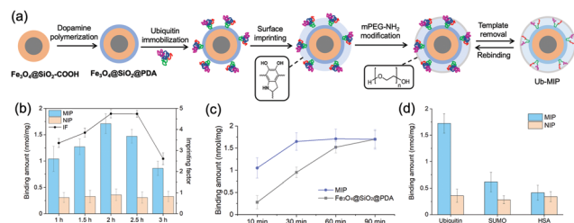
Fig. 3 (a) Schematic illustration of construction of nano receptors for ubiquitin by surface imprinting over uniformly oriented templates on PDA preformed over silica coated magnetic nanoparticles (SiMNPs). (b) Binding amounts of ubiquitin on MIP and NIP NPs synthesized at different imprinting time and modified with mPEG-NH _2 at 25 mg mL ^{-1} . (c) Comparison of the binding kinetics of ubiquitin on MIP NPs and Fe _3\text{O}_4 @SiO _2 @PDA. (d) Selectivity test results of the MIP towards ubiquitin. The concentrations of MIP NPs and the tested proteins are 0.2 mg mL ^{-1} and 0.4 \mu\text{M} , respectively.
