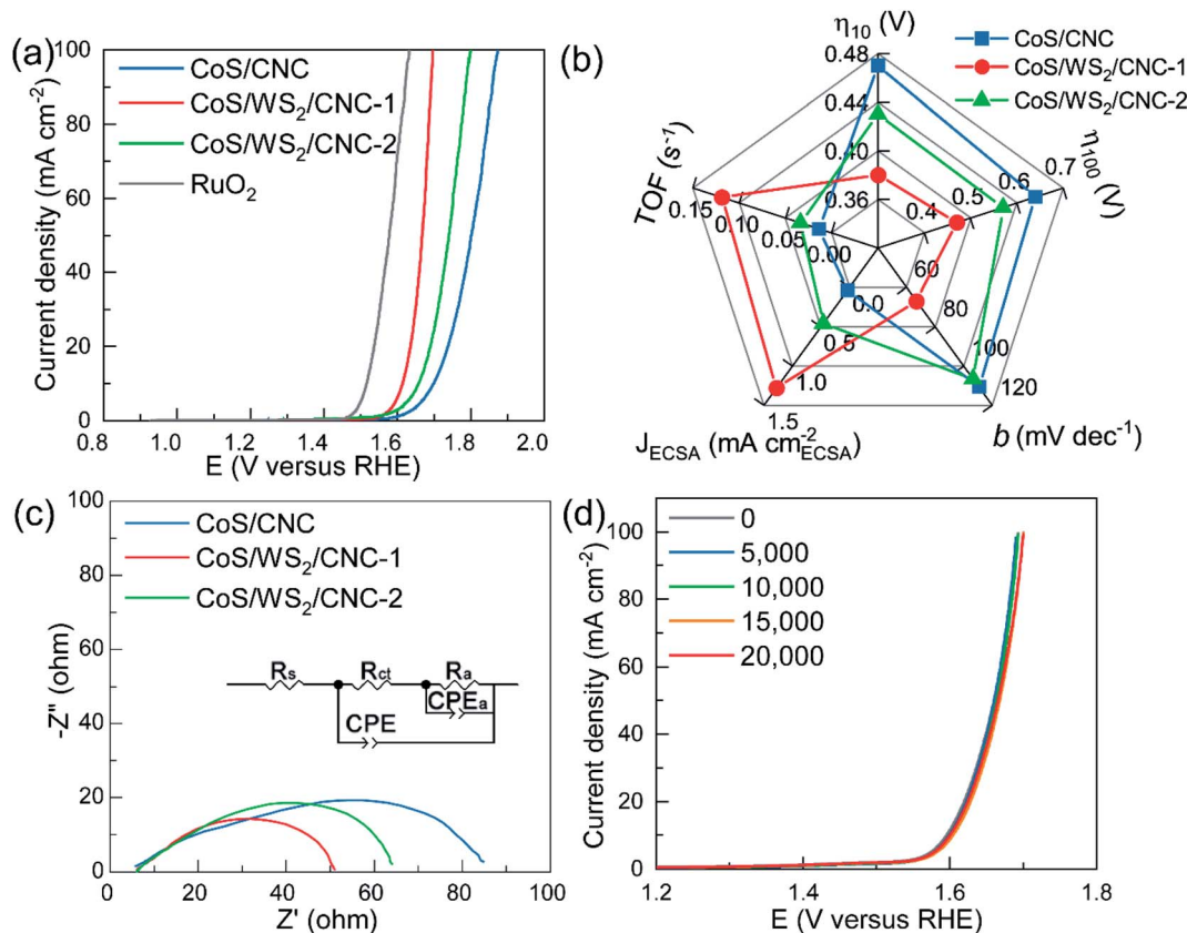
Fig. 4 Electrochemical performance towards the OER performed on an L-type glassy carbon electrode. (a) OER polarization curves at 5 \text{ mV s}^{-1} and with 85% -iR correction. (b) Summaries of an OER overpotential at 10 \text{ mA cm}^{-2} ( \eta_{10} ) and 100 \text{ mA cm}^{-2} ( \eta_{100} ), Tafel slope ( b ), an OER current at 1.65 \text{ V} versus RHE normalized by the ECSA ( J_{\text{ECSA}} ), as well as the turnover frequency (TOF) at 1.65 \text{ V} versus RHE. (c) EIS curves at 1.65 \text{ V} versus RHE (inset: corresponding equivalent circuit diagram). (d) OER polarization curves of CoS/WS 2 /CNC-1 catalyst that has been scanned from 1.4 to 1.7 \text{ V} versus RHE for 0–20 000 cycles.
