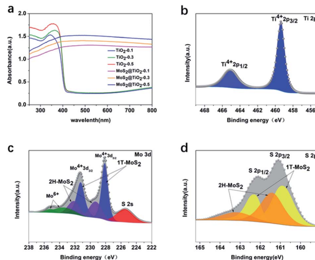
Fig. 3 UV-vis spectra of \text{TiO}_2\text{-0.5} and \text{MoS}_2\text{@TiO}_2\text{-0.5} using (a) front-illumination mode, XPS spectra of (b) Ti 2p from \text{TiO}_2\text{-0.5} , and XPS spectra of (c) Mo 3d and (d) S 2p from \text{MoS}_2\text{@TiO}_2\text{-0.5} .
