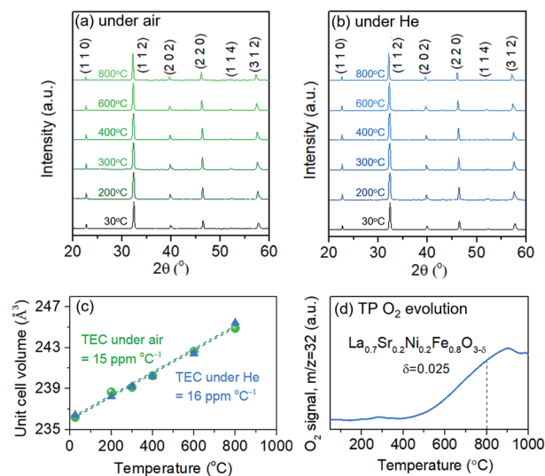
Fig. 2 In situ XRD patterns of LSNF powders at various temperatures from 30 \text{ }^\circ\text{C} to 800 \text{ }^\circ\text{C} under (a) air and (b) helium environment, (c) thermal expansion coefficient of the LSNF powders under air and helium environment, (d) temperature-programmed \text{O}_2 evolution of the LSNF powder under helium environment. \delta represents the created oxygen vacancy per formula unit of LSNF from room temperature to 800 \text{ }^\circ\text{C} .
