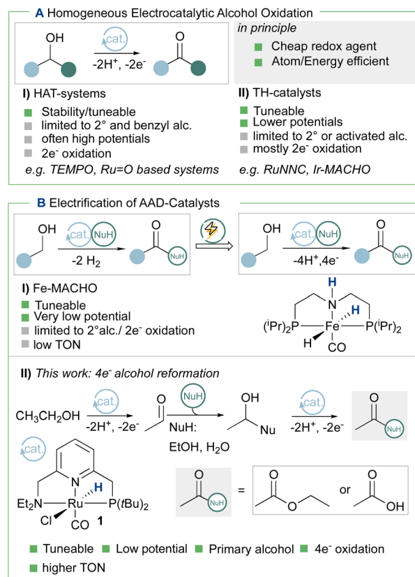
Scheme 1 (A) Advantages/limitation of electrocatalytic homogeneous alcohol oxidation using well-defined catalysts. (B) Current efforts to electrify acceptor-less alcohol dehydrogenation (AAD) systems due to their large range of application in thermal catalysis.
