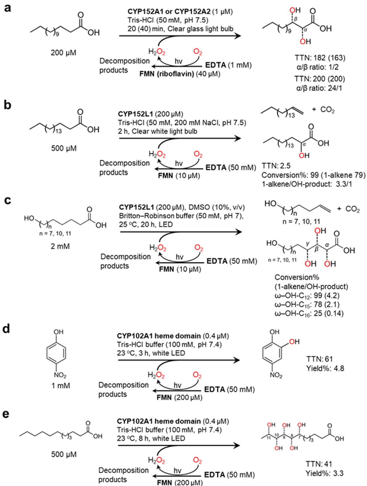
Fig. 5 Photochemically driving P450 peroxigenases using FMN as a photocatalyst and EDTA as an electron donor. Hydroxylation of fatty acids 101–103 (a and b) and \omega -hydroxylated fatty acids 104 (c) is catalyzed by CYP152 peroxigenases. CYP102A1 heme domain also shows peroxigenase activity towards 4-nitrophenol (d) and lauric acid (e). 12
