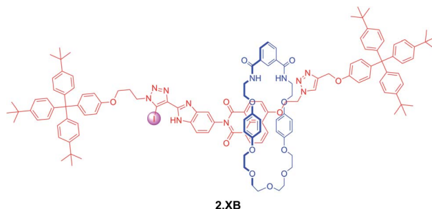
Fig. 7 XB [2]rotaxane molecular shuttle 2.XB for colorimetric anion sensing in \text{CHCl}_3 . Only in the presence of a coordinating \text{Cl}^- anion as well as acid-induced protonation of the benzimidazole does the macrocycle shuttle towards the XB anion binding site, resulting in a disruption of the hydroquinone–NDI charge-transfer interaction and a concomitant loss of colour.
