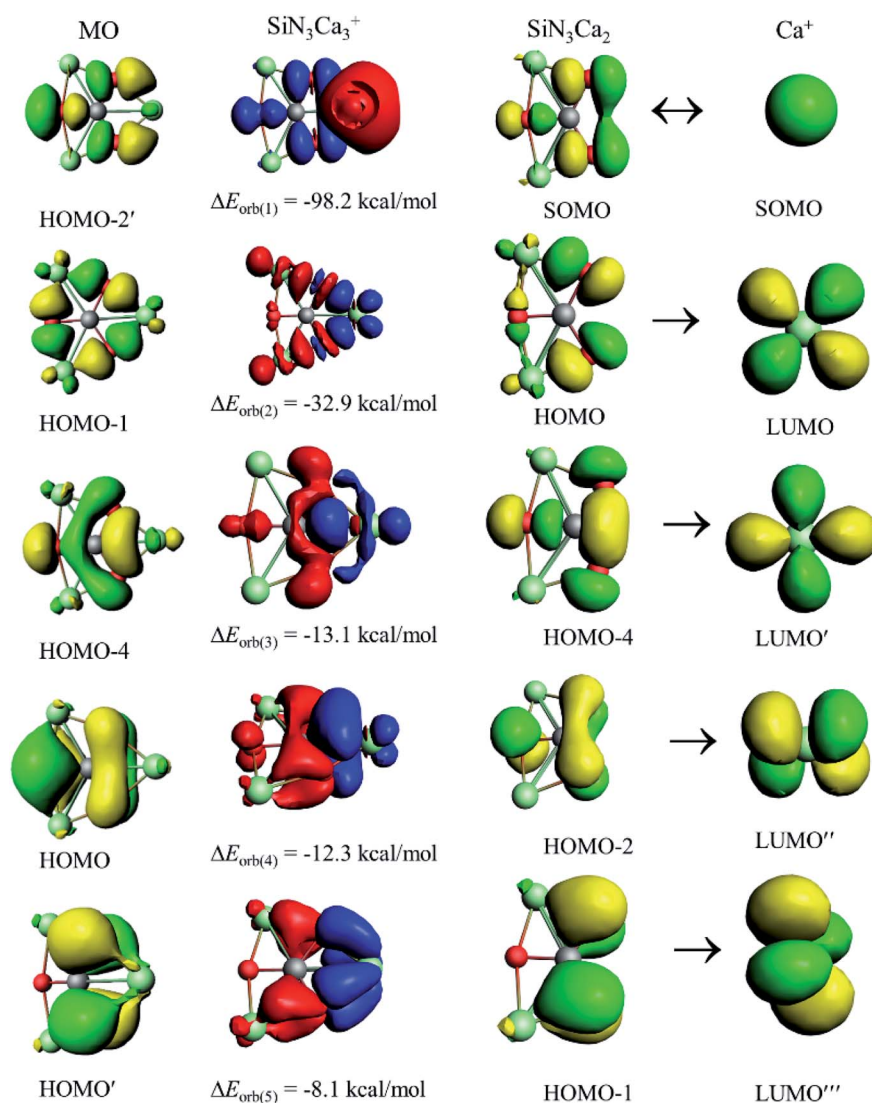
Fig. 3 Plot of the deformation densities, \Delta\rho_{(1)-(5)} corresponding to \Delta E_{\text{orb}(1)-(5)} and the related interacting orbitals of the fragments in the \text{SiN}_3\text{Ca}_3^+ cluster at the PBE0/TZ2P-ZORA//PBE0/def2-TZVP level. The orbital energy values are in \text{kcal mol}^{-1} . The charge flow of the deformation densities is from red to blue. The isovalue for \Delta\rho_{(1)} is 0.001 au and for the rest is 0.0005 au.
