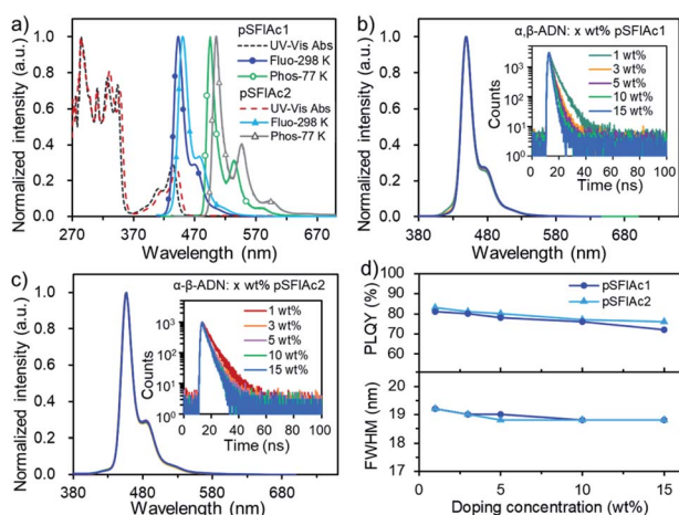
Fig. 2 (a) The absorption (left axis), fluorescence and phosphorescence (right axis) spectra of pSFIAC1 and pSFIAC2 in toluene ( 10^{-5} M). (b and c) The PL spectra and transient PL (inset) curves with different concentrations in \alpha,\beta -ADN: x wt% MR emitters ( x = 1, 3, 5, 10, 15 ). (d) The PLQYs and FWHMs of the doped films with different concentrations in \alpha,\beta -ADN: x wt% MR emitters ( x = 1, 3, 5, 10, 15 ).
