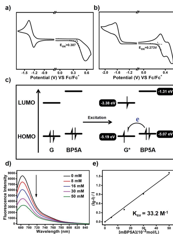
Fig. 4 Cyclic voltammogram of (a) G and (b) BP5A in DCM with 0.1 M ( n -Bu) 4 N + PF 6 - as the supporting electrolyte, Ag/Ag + as the reference electrode, a glassy-carbon electrode as the working electrode and a Pt wire as the counter electrode; scan rate, 100 mV s -1 ; Fc/Fc + was used as an external reference. (c) Schematic diagram of the electron transfer process between G and BP5A through HOMO and LUMO energy levels. (d) The emission spectra of G (1.0 × 10 -5 M) at 25 °C in acetonitrile with increasing amounts of BP5A (0–50 mM) under excitation at 650 nm. (e) The Stern–Volmer plots for the fluorescence quenching of G by BP5A in acetonitrile at 25 °C ( I 0 is the fluorescence intensity of G in the absence of BP5A and I is the fluorescence intensity in the presence of BP5A at the different concentrations ranging from 8 mM to 50 mM).
