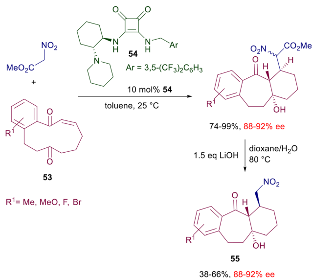
Scheme 39 Asymmetric tandem conjugate addition/aldol reaction catalyzed by squamide 54 .
