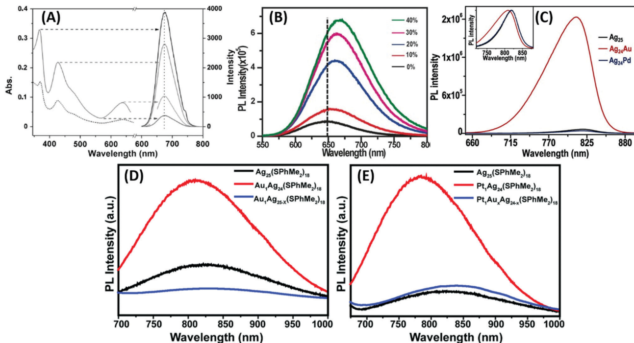
Fig. 25 (A) Enhancement in PL intensity of product NC II [Ag_{13}Au_{12}(PPh_3)_{10}(SR)_5Cl_2]^{2+} . PL (—), UV/Vis (· · ·), UV/Vis and excitation spectra (left), and emission spectra (right) at arrow-indicated excitation wavelengths. (B) PL spectra of undoped Ag_{25} and different percentages (mmol%) of Au-doped Ag_{25} clusters. (C) PL spectra of [Ag_{25}(SPhMe_2)_{18}]^- , [Ag_{24}Au(SPhMe_2)_{18}]^- , and [Ag_{24}Pd(SPhMe_2)_{18}]^{2-} clusters. Inset represents the normalized spectra. PL spectra of (D) Ag_{25}(SPhMe_2)_{18} , Au_1Ag_{24}(SPhMe_2)_{18} , and Au_xAg_{25-x}(SPhMe_2)_{18} and (E) Ag_{25}(SPhMe_2)_{18} , Pt_1Ag_{24}(SPhMe_2)_{18} , and Pt_1Au_xAg_{24-x}(SPhMe_2)_{18} with \lambda_{ex} = 405 nm. (A)–(C) Reproduced with permission. 135,138,237 Copyright 2014. Wiley-VCH. (D) and (E) reproduced from ref. 143 with permission from The Royal Society of Chemistry, Copyright 2014.
