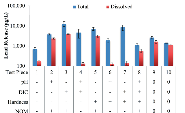
Fig. 2 Total and dissolved lead release from the test pieces. Total lead was measured from the weekly composite samples over the entire 20 week study. Dissolved lead was measured from the samples collected after the final 48 hour stagnation event in weeks 4, 8, 10, 12, 14, 16, 19 and 20. Bars represent average values and error bars represent the 90% confidence intervals.
