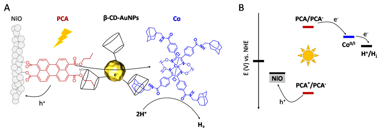
Fig. 1 (A) Representation of the PCA| \beta -CD-AuNPs|Co supramolecular assembly anchored onto a mesoporous NiO thin film, (B) energy diagram of the photocathode.
