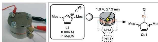
Fig. 1 Miniaturised electrochemical flow reactor comprising circular stacked electrodes (48 mm diameter) separated by PTFE spacers (1 mm thick) with flow channels of 0.464 mL. Model reaction; synthesis of Cu1 from L1 and copper electrodes.
