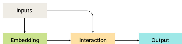
Fig. 2 High-level architecture of the models.
