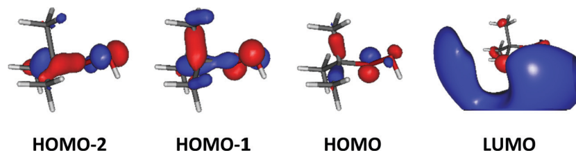
Fig. 6 Outermost molecular orbitals of t BuOOH as computed at the HF/aug-cc-pVTZ level.
