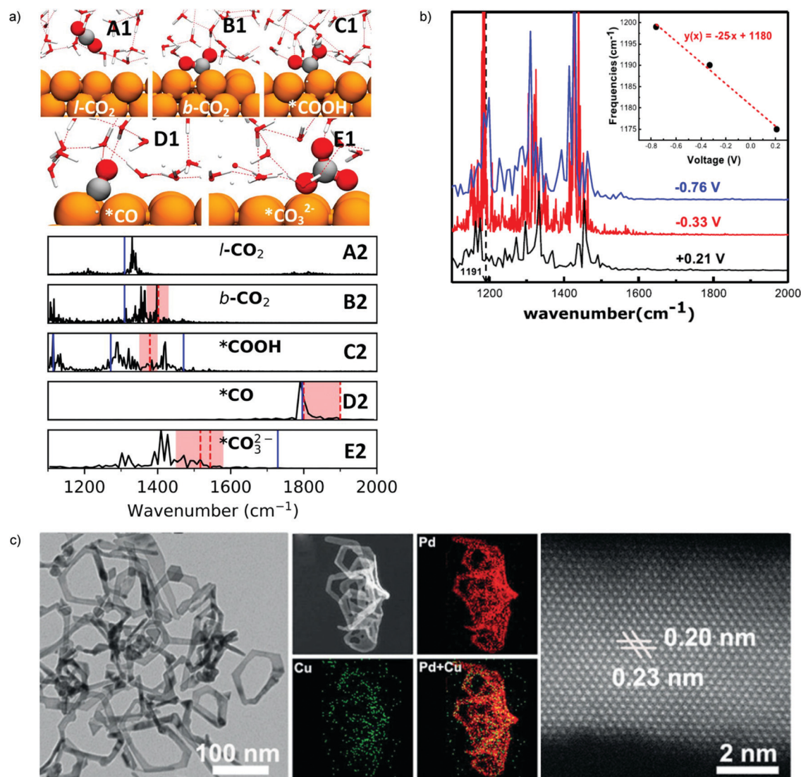
Fig. 9 (a) Snapshots of the structures and v-DoS \text{CO}_2 ( \text{l-CO}_2 ), chemisorbed \text{CO}_2 ( \text{b-CO}_2 ), \text{*COOH} , \text{*CO} , and \text{*CO}_3^{2-} from o-QM-MD simulations and 2PT analysis. The color codes are Cu in orange, O in red, C in silver, and H in white. The hydrogen bonds are shown as dashed red lines. In bottom part, v-DoS from o-QM-MD is shown as a solid black line, the experimental frequencies are shown as a red dashed line, and the vibrational frequencies from v-QM optimization are shown as solid blue lines for comparison. ( \text{l-CO}_2 and \text{b-CO}_2 are the same from v-QM, because \text{b-CO}_2 is unstable in vacuum and automatically converts to \text{l-CO}_2 after optimization.) (b) The simulated potential-dependent v-DoS of \text{*HOC-COH} at +0.21 V, -0.33 V, and -0.76 V. Inset shows the blue shift of the 1191\text{ cm}^{-1} peak (a feature of C–O stretch of C–OH) as a function of applied potential. (c) Characterization of Pd/Cu NRs. From left to right: TEM image; HAADF-STEM image and the corresponding STEM-EDX elemental mapping; atomic resolution HAADF-STEM image. (a) and (b) are adapted with permission from ref. 187, (c) is adapted with permission from ref. 181, Copyright 2017 Wiley-VCH Verlag GmbH & Co. KGaA, Weinheim.
