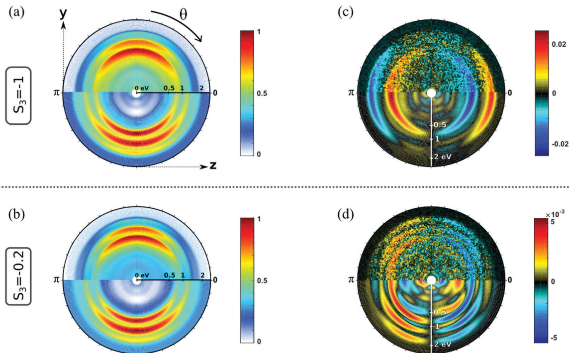
Fig. 3 Normalized photoelectron angular distribution (PAD) of S -(+)-fenchone photoionized at 358 nm by (a) a circularly polarized field ( S_3 = -1 ) and (c) its corresponding antisymmetric signal, i.e. PECD. Upper half of each image is raw experimental data, that have been antisymmetrized with respect to the light propagation direction z . Lower half of each image is Abel inverted image. (b and d) are the same as (a and c) for a lower ellipticity ( S_3 = -0.2 ). The PAD are normalized by their maximal amplitudes (pixel value) which are also employed to normalize the PECD and PEELD images.
