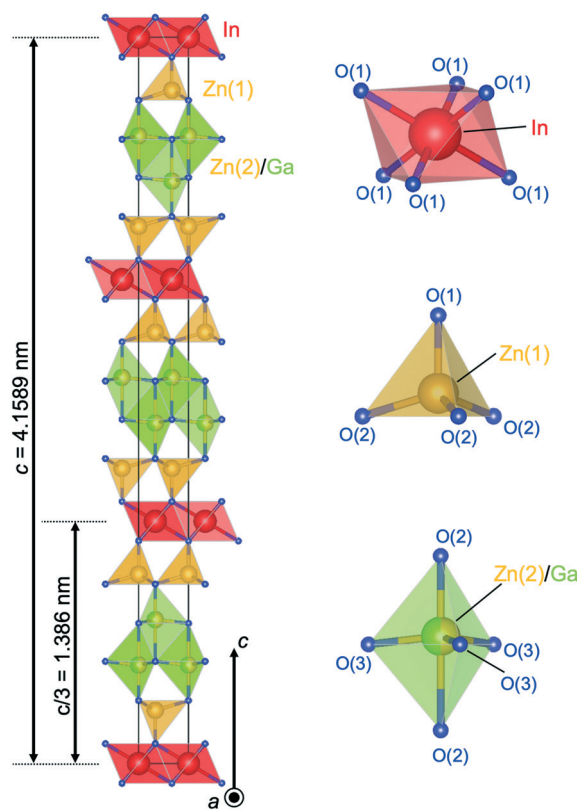
Fig. 6 Crystal structure of \text{InGaO}_3(\text{ZnO})_3 . Coordination of \text{InO}_6 is octahedra, \text{Zn}(1)\text{O}_4 is tetrahedra, and \text{Zn}(2)/\text{GaO}_4 is trigonal bipyramid.
