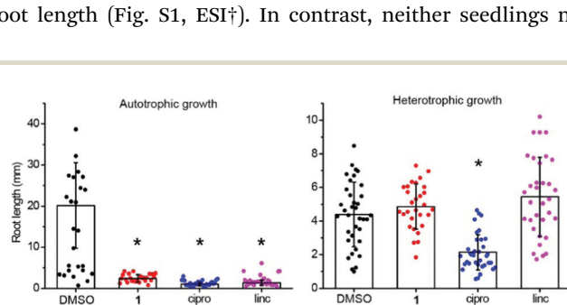
Fig. 2 Linezolid 1 is inactive against dark-grown plants. Linezolid 1 was active in autotrophic (“auto”, no glucose in growth media, under light), but not heterotrophic (“hetero”, glucose in growth media, no light) growth regimes; ciprofloxacin (cipro), which does not directly affect chloroplast translation, was used as a positive control and inhibited plant growth in both conditions; lincomycin (linc), which inhibits chloroplast translation, was active only in autotrophic conditions.
