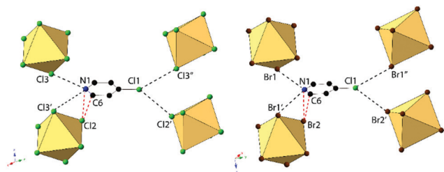
Fig. 4 Local structure of isomorphous compounds 2 (left) and 6 (right) showing halogen and hydrogen bonding (black) between [TeX 6 ] 2- octahedra and the halogen substituent on the pyridinium. Also shown is the short X...N/C contacts between the protonated nitrogen N1 and carbon C6 and the metal bound halide Cl2 (red).
