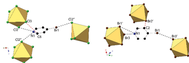
Fig. 6 Local structure of 3 (left) and 7 (right) showing hydrogen and halogen bonding (black dashed lines). Short X...C contacts shown as red dashed lines. Compound 7 assumes a different packing scheme and space group ( P1 vs. P2(1)/c ) from compound 3 .
