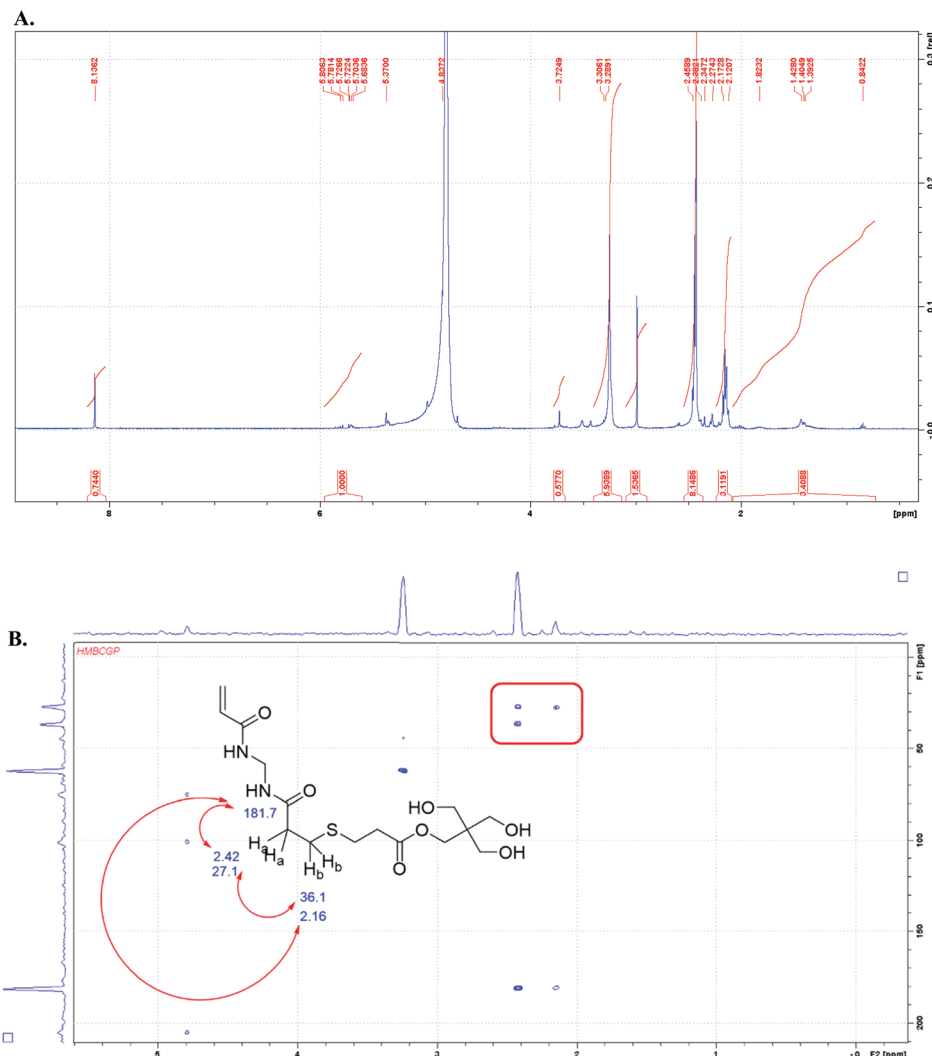
Fig. 2 The NMR analysis for 1:1 (thiol:ene) gel after basic degradation with sodium hydroxide in deuterium oxide solvent ( \text{D}_2\text{O} , 400 MHz): (A) the ^1\text{H} NMR spectrum of the hydrolysis product; (B) the gHMBC spectrum for the hydrolysis product with key correlations highlighted.
