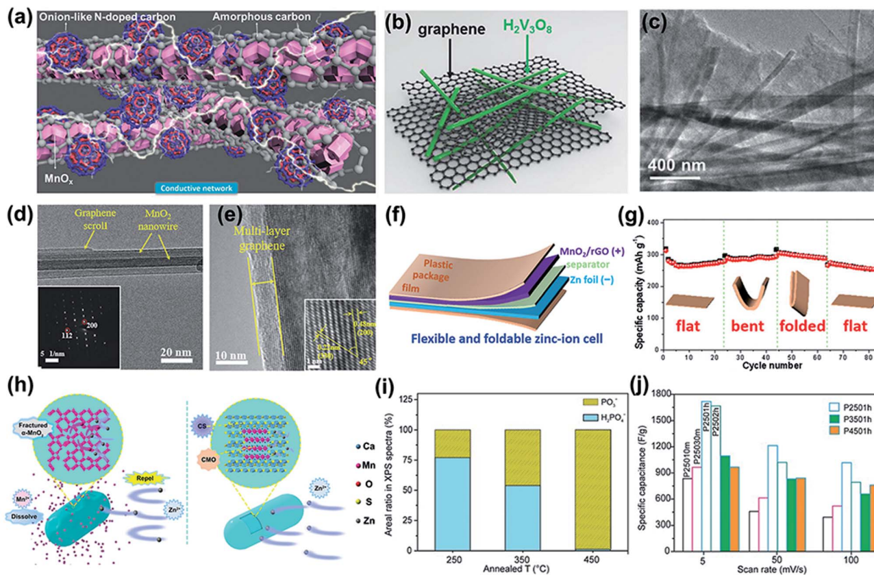
Fig. 8 (a) Schematic of the structure of \text{MnO}_x@N-C nanorods. Reproduced with permission. 117 Copyright 2018, Wiley. (b) Schematic illustration of the structure of \text{H}_2\text{V}_3\text{O}_8 NW/graphene. (c) TEM image of \text{H}_2\text{V}_3\text{O}_8 NWs on graphene films. (b and c) Reproduced with permission. 51 Copyright 2018, Wiley. (d) TEM images and SAED (inset) of \alpha\text{-MnO}_2 /graphene scrolls. (e) The HRTEM of \alpha\text{-MnO}_2 /graphene scrolls. (d and e) Reproduced with permission. 126 Copyright 2018, Wiley. (f) Schematic illustration of a flexible and foldable ZIB cell. (g) Cycling stability of the ZIB cell under different mechanical deformations. (f and g) Reproduced with permission. 129 Copyright 2020, Wiley. (h) The battery reaction mechanism schematic diagram of \alpha\text{-MnO}_2 and \text{Ca}_2\text{MnO}_4 . Reproduced with permission. 131 Copyright 2019, American Chemical Society. (i) Area% change of \text{H}_2\text{PO}_4^- and \text{PO}_3^- at the surface of PCO as a function of annealed temperature. (j) Specific capacitances of different PCO samples prepared under various conditions as a function of scan rate. (i and j) Reproduced with permission. 132 Copyright 2016, Wiley.
