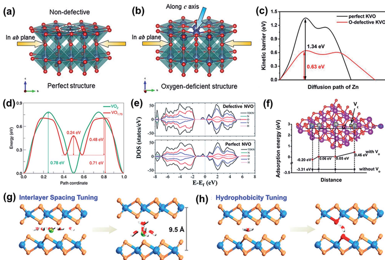
Fig. 5 Structure of (a) p-VO and (b) O_d -VO. (a and b) Reproduced with permission. 98 Copyright 2019, Wiley. (c) Calculated diffusion barriers for paths in perfect KVO and O -defective KVO. Reproduced with permission. 101 Copyright 2019, Wiley. (d) Calculated Zn ion diffusion energy barriers in VO_2 and VO_{1.75} . Reproduced with permission. 99 Copyright 2020, American Chemical Society. (e) The projected density of states (PDOS) and the total density of states (TDOS) of defective and perfect NVO. Reproduced with permission. 93 Copyright 2020, Royal Society of Chemistry. (f) The calculated adsorption energies for Zn^{2+} on the surfaces of perfect \sigma - MnO_2 and \sigma - MnO_2 with oxygen vacancies. Reproduced with permission. 102 Copyright 2019, Wiley. (g) Schematic illustration of interlayer expanded MoS_2 . (h) Schematic illustration of hydrophilicity tuning. (g and h) Reproduced with permission. 103 Copyright 2019, American Chemical Society.
