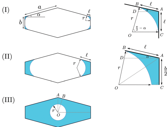
Fig. 3 Three scenarios of the wetting liquid in the cross-section of a nearly-rectangular channel. (I) The liquid–vapor interfaces form four separated arcs in the corners. (II) The liquid–vapor interfaces form two separated arcs in the corners, with the b side is fully covered by the fluid. (III) The liquid–vapor interface is a full circle, with the perimeter of the cross-section all covered by the fluid.
