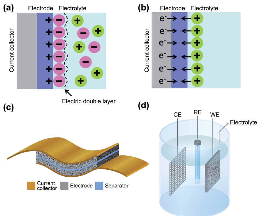
Fig. 1 Scheme of (a) an electric double-layer capacitor and (b) a pseudocapacitor. (c) Schematic drawing of an assembled supercapacitor with a sandwich structure showing current collectors, electrodes and the separator, as used in two-electrode measurements. (d) Schematic drawing of a three-electrode measurement set-up showing a reference electrode, a Pt mesh as the counter electrode and one supercapacitor electrode as the working electrode, all immersed in the electrolyte.
