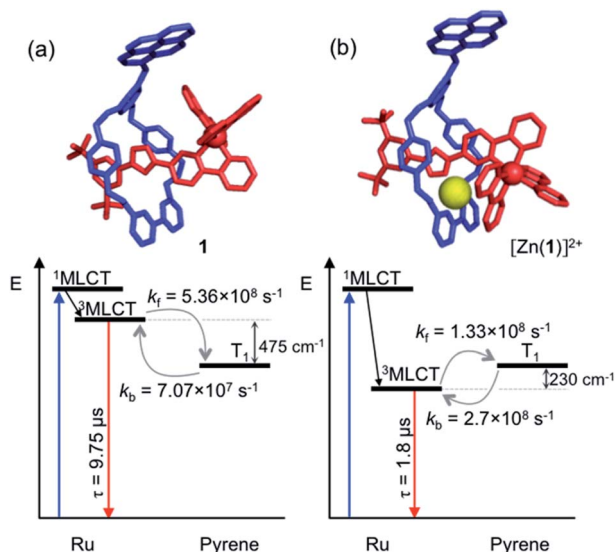
Fig. 5 Jablonski–Perrin diagram representing pertinent low lying excited states and electronic energy transfer between ^3\text{MLCT} and triplet pyrene of rotaxanes 1 (a) and [\text{Zn}(1)]^{2+} (b) at 300 K. Molecular modelling of rotaxane structures used Spartan'18 – MMFF force field. 19
