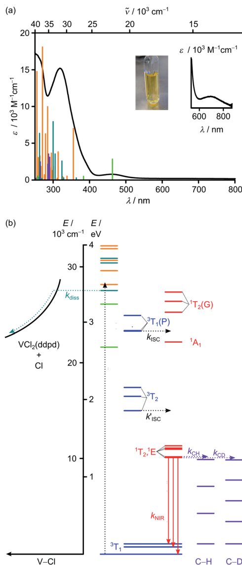
Fig. 1 (a) Absorption spectrum including a zoom into the red spectral region (black) and photograph of VCl_3(ddd-p-[D_0]) in CH_3CN . The vertical bars correspond to spin-allowed CT transitions calculated by TDDFT-UKS (hypsochromically shifted by 3400\text{ cm}^{-1} ). The colour code of the vertical bars indicates the major character of the transition as ddd-p \rightarrow V ^3LMCT (light green), Cl \rightarrow V ^3LMCT (petrol green), ILCT (orange) and V \rightarrow ddpd ^3MLCT (purple). (b) Jablonski diagram constructed from TDDFT-UKS ( ddd-p \rightarrow V ^3LMCT (light green), Cl \rightarrow V ^3LMCT (petrol green) and ILCT (orange)) and CASSCF-NEVPT2 calculations ( ^3MC states in blue; ^1MC states in red). Notation of MC states is according to octahedral symmetry. ISC = intersystem crossing; diss = V–Cl homolysis; NIR = NIR emission; C–H and C–D overtones in purple = multiphonon relaxation (experimental overtone energies from ref. 34).
