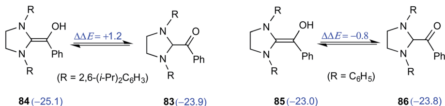
Scheme 18 The relative energies of the enol and keto (shown in parentheses, in kcal mol -1 ) variants of the Breslow intermediate with different aryl groups on the nitrogen atoms of imidazolyliene carbene.
