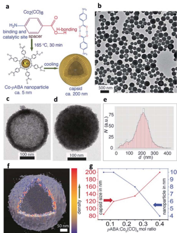
Fig. 2 (a) Synthesis of CoNPs using \text{Co}_2(\text{CO})_8 and p ABA in 1,2-DCB and their spontaneous self-assembly into shell-like capsids; (b) Transmission Electron Microscopy (TEM) images showing spherical capsids for \text{Co}_2(\text{CO})_8 / p ABA. Capsids with less (c) and more (d) kinetically trapped p ABA in the interior; (e) size distribution of capsids; (f) Electron Tomography (ET) reconstruction resolves clearly the CoNP shell layer from the hollow interior; (g) NP and capsid sizes are tuned by their composition. Reproduced with permission from ref. 50. Copyright 2017 Wiley and Sons.
