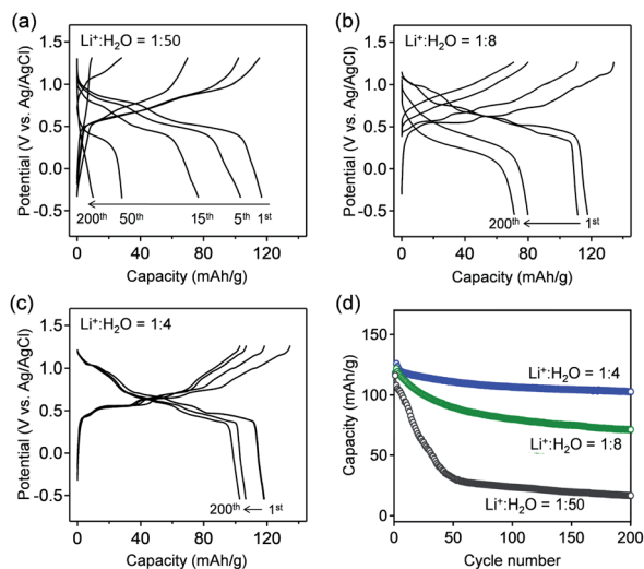
Fig. 3 Charge/discharge curves of VOPO 4 ·H 2 O electrodes with aqueous Li + electrolytes. The Li + : H 2 O ratios are (a) 1 : 50 (LiTFSI/50H 2 O), (b) 1 : 8 (LiTFSI/8H 2 O), and (c) 1 : 4 (LiTFSI/4H 2 O), respectively. The specific current is 1 A g -1 . (d) Capacity retention during 200 charge/discharge cycles.
