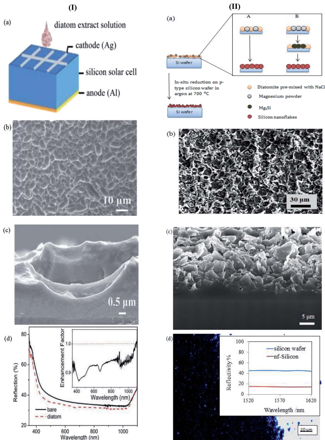
Fig. 12 Schematic illustration of the 2 approaches reported to suppress surface reflectivity of silicon based solar cell (I) (a) schematic illustration of synthesis process (b) and (c) SEM images diatom extract (d) surface reflectivity of diatom extract 71 and (II) (a) schematic illustration of synthesis process (b) and (c) SEM images of silicon nanoflakes (d) surface reflectivity of silicon nanoflakes. 112
