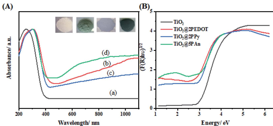
Fig. 6 (A) UV-Vis diffuse reflectance spectra of (a) \text{TiO}_2 , (b) \text{TiO}_2@2\text{PEDOT} , (c) \text{TiO}_2@2\text{PPy} , and (d) \text{TiO}_2@5\text{PAn} , (B) plots of transformed KM function.
