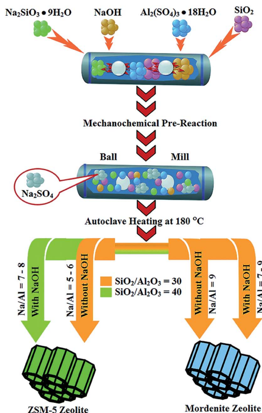
Scheme 1 Graphical summary of key reactions steps used. 33
