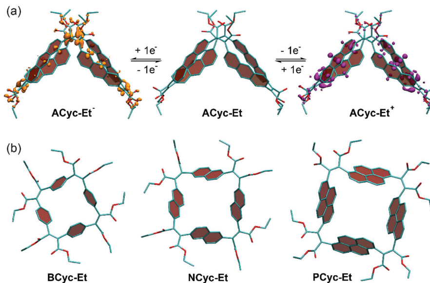
Fig. 4 Calculated conformation of (a) ACyc-Et in the neutral and singly charged states and (b) BCyc-Et , NCyc-Et , and PCyc-Et in the neutral state. Panel (a) shows electron density differences between the neutral and charged states (isovalues -0.0015e for ACyc-Et − and +0.0015e for ACyc-Et + ). Hydrogen atoms omitted for clarity.
