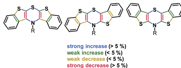
Fig. 3 Relative change of Wiberg bond orders \Delta(\text{BO}_{x+} - \text{BO}_x) from neutral precursors 5, 6, and 7 to radical cations 5 + , 6 + , and 7 + in the BBTT core (R = p -fluorophenyl; uB3LYP/6-311G**) (A detailed list of bond orders is given in the ESI†).
