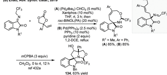
Scheme 87 [5 + 3]-Cycloaddition towards 8-membered spiroindolones.
