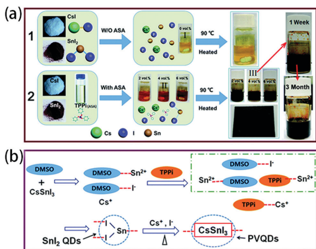
Fig. 7 (a) Schematic of the preparation process of CsSnI 3 QD solution prepared with and without TPPI and the stability of the QD solution stored for different periods. (b) Scheme of the PVQD production process. 40 Copyright 2019, Royal Society of Chemistry.
