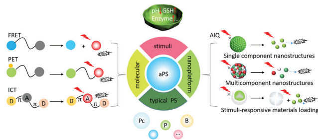
Scheme 1 Schematic illustration of design strategies including molecular and nanoplatform structures, stimuli and typical PSs for aPSs. B is Boron-dipyrrromethene, Pc is phthalocyanine and P is porphyrin.
