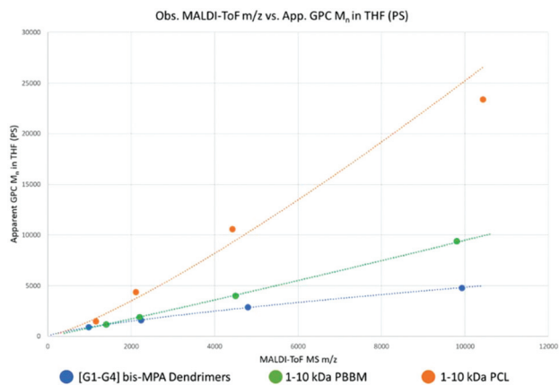
Fig. 3 Observed m/z by MALDI-ToF MS versus apparent M_n by GPC (calibrated against PS standards) using the M_n values from Table 1.
